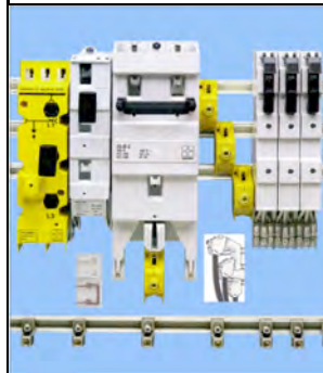
RAILS & CLAMES ISOLES
